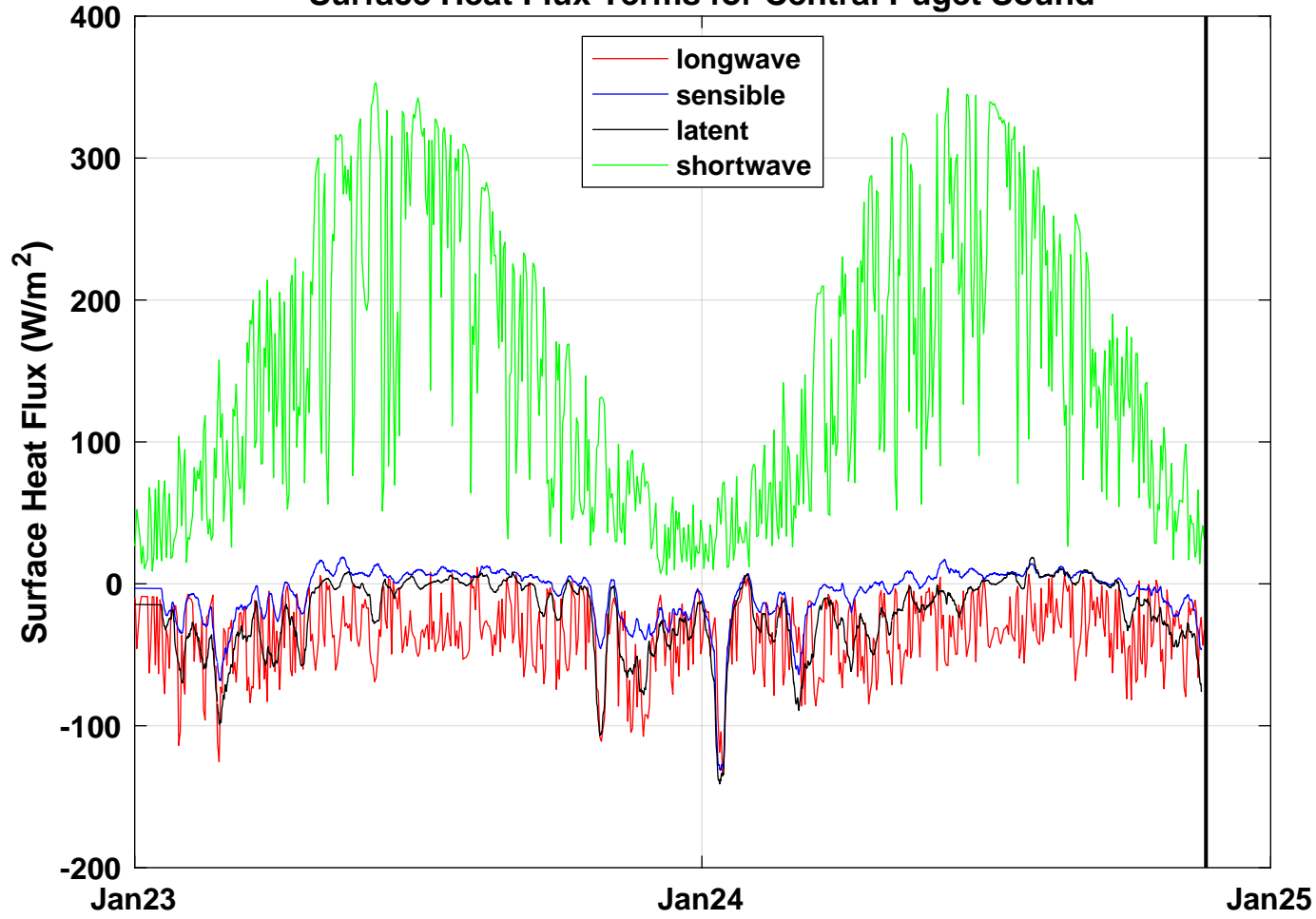
Surface Heat Flux Terms for Central Puget Sound
